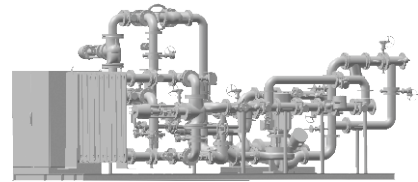
Large integrated submerged liquid cooling unit
