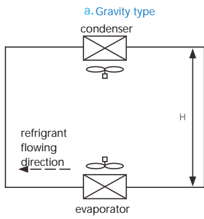
Heat pipe backplane air conditioner -PHE application
