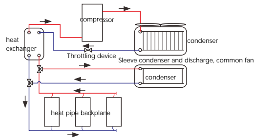
Schematic diagram of the air conditioner + heat pipe backplane in the dual-source integrated equipment room-PHE application
