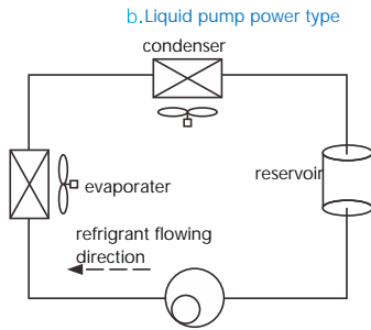
Three separate heat pipe-PHE applications (condenser)
