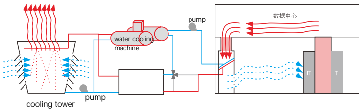
Principle of total solution for cold water production by direct evaporative cooling - PHE application
