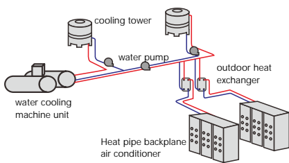
Heat pipe backplane air conditioner -PHE application
