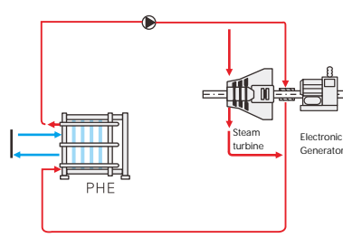
PHE application in lubricating oil cooling of steam turbine
