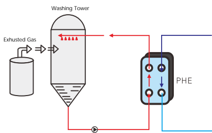
PHE application in heat recovery of washing tower
