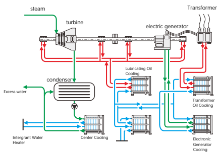
PHE application in power plant
