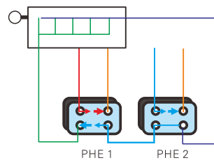
PHE application in diesel oil cooling
