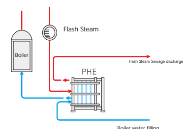
PHE application in heat recovery
