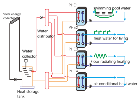
Application of plate heat exchanger in solar energy collection system
