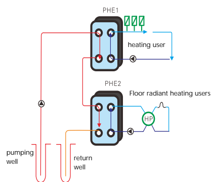
Application of plate heat exchanger in geothermal system
