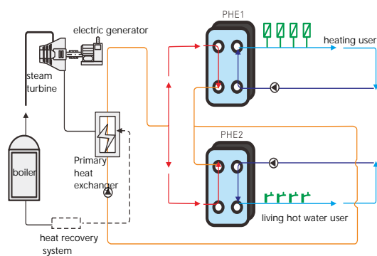
Application of plate heat exchanger in central heating system
